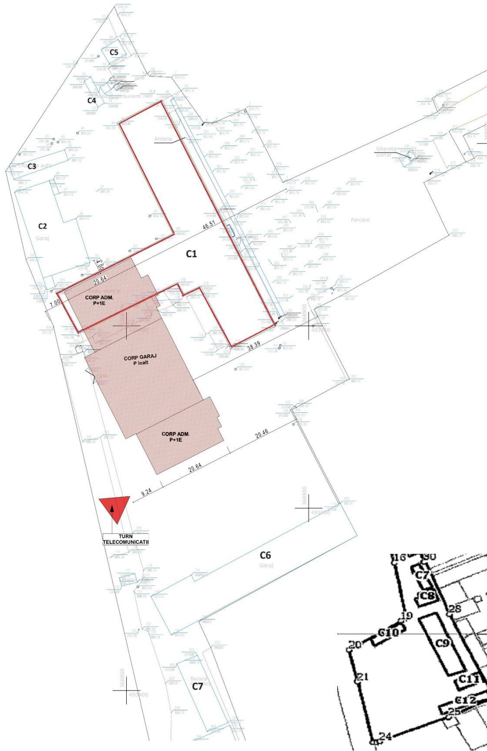
Figure 3 Site layout - Proposed location of the new building (drawn in pink) on the site and the existing buildings. The Building C1 that will be demolished under the Project is lined in red
